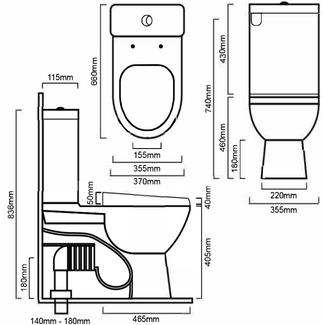
WCKENT: 370mm x 660mm x 836mm
